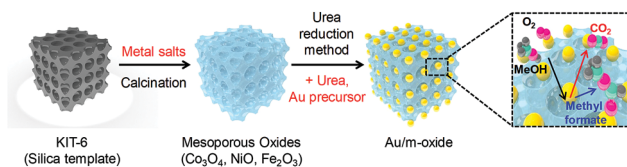
Fig. 1 Schematic diagram of the hard-templating (nanocasting) approach for the preparation of mesoporous oxide supported Au nanoparticle catalysts.
