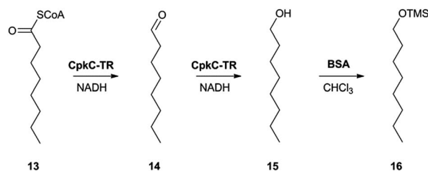
Scheme 1 Reactions catalyzed by CpkC-TR using octanoyl-CoA 13 and octanal 14 as substrate analogues and conversion of 1-o-octanol 15 to its TMS ether 16 to facilitate GC-MS analysis.
