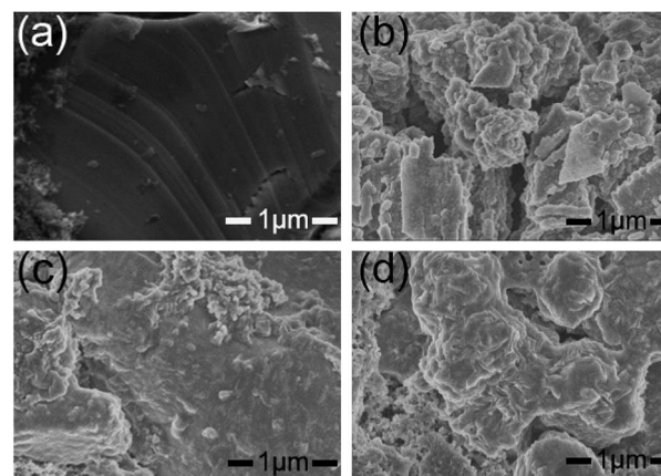
Fig. 4 (a) SEM image of pristine LiCoO 2 electrode surface. (b) With electrolyte A0 after 160 cycles; (c) with electrolyte A1 after 160 cycles; (d) with electrolyte A2 after 160 cycles.
