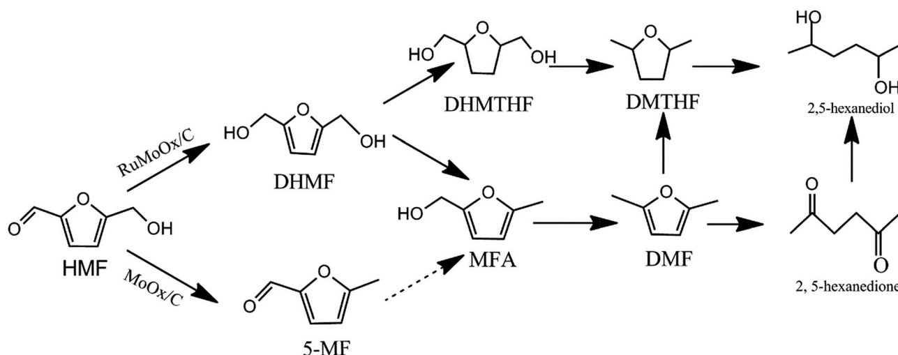
Scheme 1 Proposed reaction network for hydrogenolysis of HMF to DMF.
