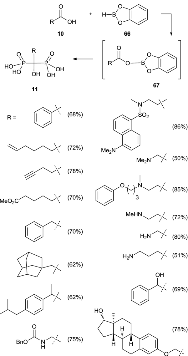
Scheme 16 Reagents and conditions: (i) THF, rt. (ii) P(OSiMe 3 ) 3 , 16 h, 25 °C; then MeOH, 2 h.
