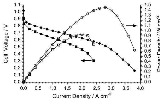
Fig. 14 The \text{H}_2/\text{O}_2 AEMFC performances at 80^\circ\text{C} of the LDPE-AEM (100 kGy) with Pt/C ( 0.4\text{ mg}_{\text{Pt}}\text{ cm}^{-2} ) (●,○) and Ag/C ( 0.8\text{ mg}_{\text{Pt}}\text{ cm}^{-2} ) (■,□) cathodes: PtRu/C (50% wt Pt and 25% wt Ru) anodes ( 0.4\text{ mg}_{\text{Pt}}\text{ cm}^{-2} loading). The 1.0 SLPM (RH = 100%) gas supplies were not pressurised.
