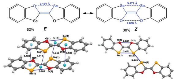
Scheme 22 Chalcogen bonding in ( E/Z )-2,2'-bibenzo[ d ][1,3]oxaselenolylidene. 140
