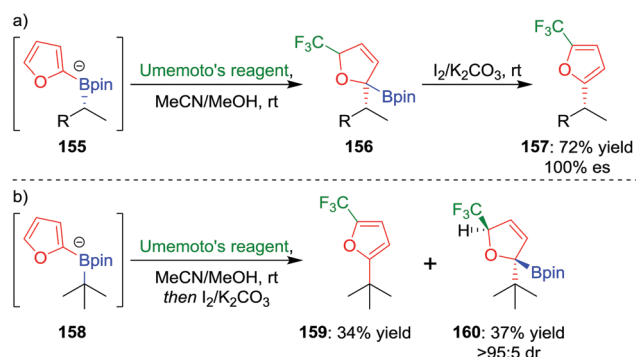
Scheme 21 Transition-metal-free three-component couplings of secondary and tertiary boronic esters with trifluoromethylated furans. R = CH 2 CH 2 C 6 H 4 OMe, Umemoto's reagent = 5-(trifluoromethyl)dibenzothio-phenium trifluoromethanesulfonate.
