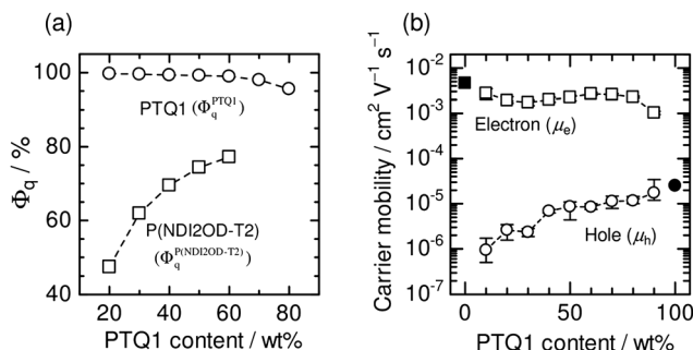
Fig. 19 (a) PL quenching efficiencies ( \Phi_q ) of PTQ1 (circles) and P(NDI2OD-T2) (squares) in PTQ1/P(NDI2OD-T2) blend films as functions of PTQ1 weight percentage. (b) Hole (open circles) and electron (open squares) mobilities in PTQ1/N2200 blend films as functions of PTQ1 weight percentage. The solid circle and square indicate the hole and electron mobilities in the PTQ1 and P(NDI2OD-T2) neat films, respectively. Reproduced with permission from (ref. 51). Copyright 2013, Wiley-VCH Verlag GmbH & Co. KGaA, Weinheim.
