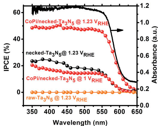
Fig. 3 IPCE of raw- \text{Ta}_3\text{N}_5 (orange), necked- \text{Ta}_3\text{N}_5 (black) and CoPi/necked- \text{Ta}_3\text{N}_5 (red) electrodes. The absorption spectrum (black solid curve) for raw \text{Ta}_3\text{N}_5 is presented for comparison.
