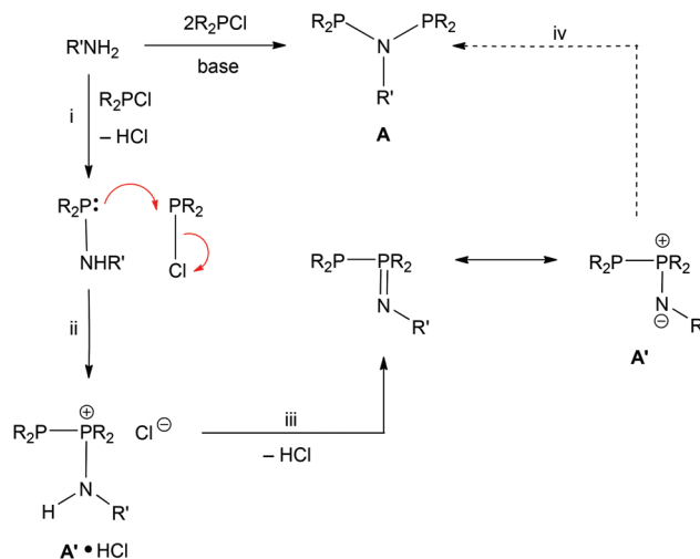
Scheme 7 Proposed pathway for the conversion of an amine to a PNP ligand. A dotted line is used for step iv since this step is not observed with the aminophobanes.
