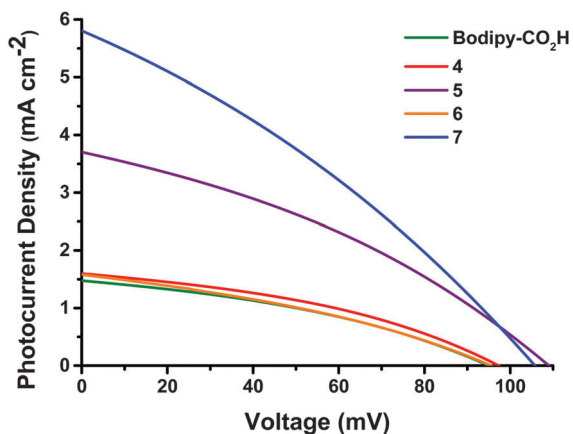
Fig. 3 Current–voltage characteristics of the dye-sensitized NiO solar cells with 0.1 M I 2 , 1.0 M Lil electrolyte and 4 (red), 5 (purple), 6 (orange), 7 (blue) and Bodipy-CO 2 H (green) under AM 1.5G (100 mW cm -2 ) illumination.
