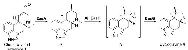
Fig. 1 Aj_EasH catalytic reaction to generate cycloclavine 4 .
