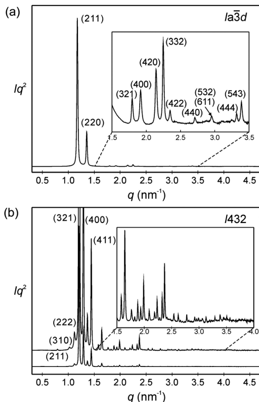
Fig. 3 SAXS diffractograms of (a) the Cub/ Ia\bar{3}d phase ( a_{\text{cub}} = 13.10 nm) of AB8 , recorded at T = 150 °C on heating (for wide angle scattering see Fig. S10b, ESI † ); (b) the Cub/ I432 phase ( a_{\text{cub}} = 19.46 nm) of AB14 at T = 140 °C, the curve on top is enhanced by a factor of 7 and only some diffractions at lower angles are labelled; see also Tables S3–S6 (ESI † ).
