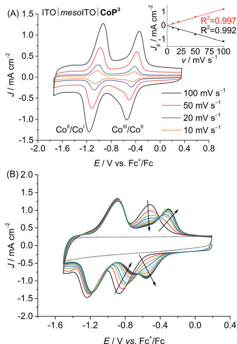
Fig. 3 (A) CVs of ITO|mesoITO|CoP 3 in DMF/TBABF 4 electrolyte (0.1 M) at different scan rates (10, 20, 50, 100 mV s -1 ). Inset: The correlation between the peak current density, J_p (Co II /Co I ), and scan rate, v , is shown. The black and red traces represent linear fits to the data points. (B) Consecutive CVs of ITO|mesoITO|CoP 3 in DMF/TBABF 4 (0.1 M) at a scan rate of 100 mV s -1 showing cathodically induced replacement of the axial bromido ligand by DMF. The background of ITO|mesoITO without catalyst is shown as dotted line. Note that ligand exchange has already occurred in the CVs shown in (A).
