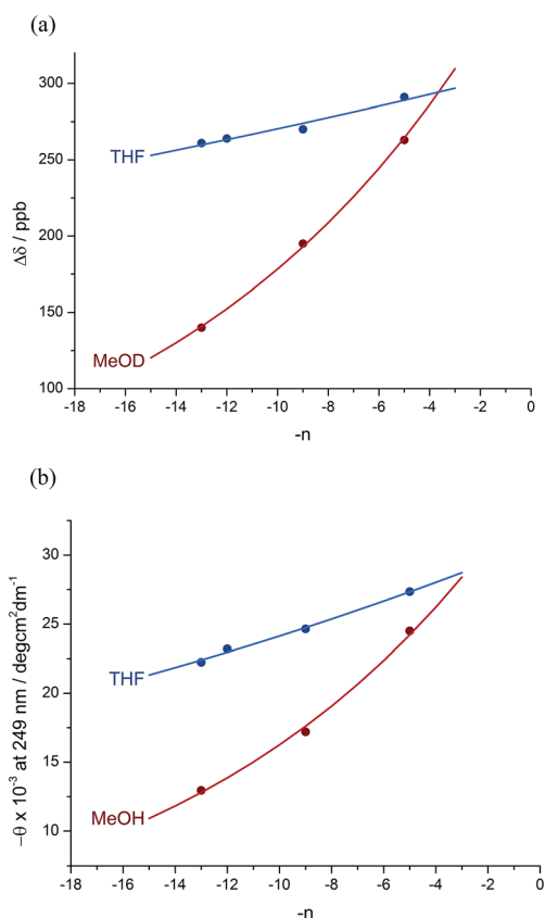
Fig. 10 Effect of chain length n on characteristic features of the products 8a-d. (a) Exponential decay of anisochronicity in the azepine CH 2 groups with chain length ( \bullet in THF at 23 °C; \bullet in methanol at 23 °C; -f = 0.013 ; \bullet in methanol at 23 °C; -f = 0.077 ); (b) exponential decay of molar ellipticity at 249 nm ( \bullet in THF at 23 °C; \bullet in methanol at 23 °C; -f = 0.025 ; \bullet in methanol at 23 °C; -f = 0.076 ).
