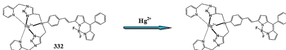
Fig. 292 Chemical structure of ligand 332 and the proposed ligand-metal binding model.
