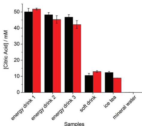
Fig. 6 Concentration of citric acid in drinks as determined by 1 H NMR spectroscopy (black bars) and by the dye 4–Al 3+ sensing ensemble (red bars). Experimental details are given in the ESI†
