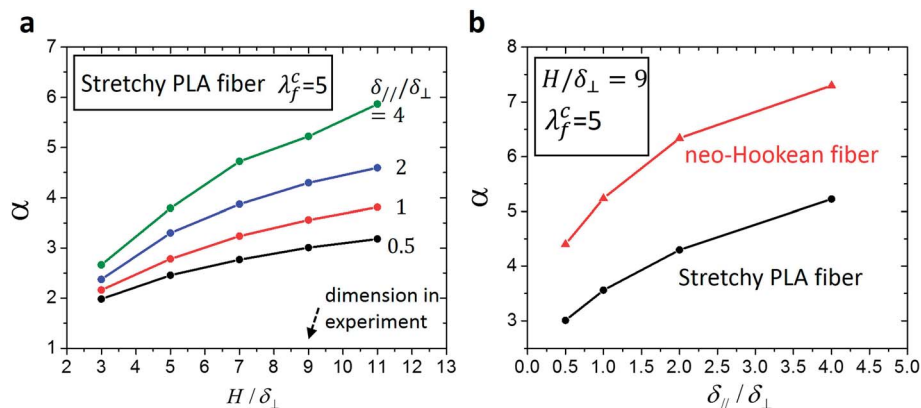
Fig. 4 The non-dimensional parameter \alpha calculated from the finite element model. (a) The calculated \alpha as functions of H/\delta_\perp and \delta_{\parallel}/\delta_\perp for the stretchy-PLA-fiber mesh used in the experiments. (b) The calculated \alpha as functions of \delta_{\parallel}/\delta_\perp for the stretchy-PLA-fiber mesh and a neo-Hookean-fiber mesh.
