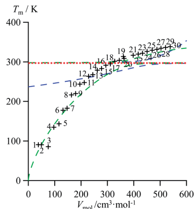
Fig. 8 Correlations between molar volumes V_{mol} and melting temperatures T_m for linear alkanes C_nH_{2n+2} ( n = 1-30 ) fitted using a parabolic H/S function (blue trace) or a reciprocal Hill plots (green trace). The horizontal dotted red trace corresponds to the asymptotic behaviour occurring when the melting temperature approaches the selected reference temperature T^0 = 298.15 K.
