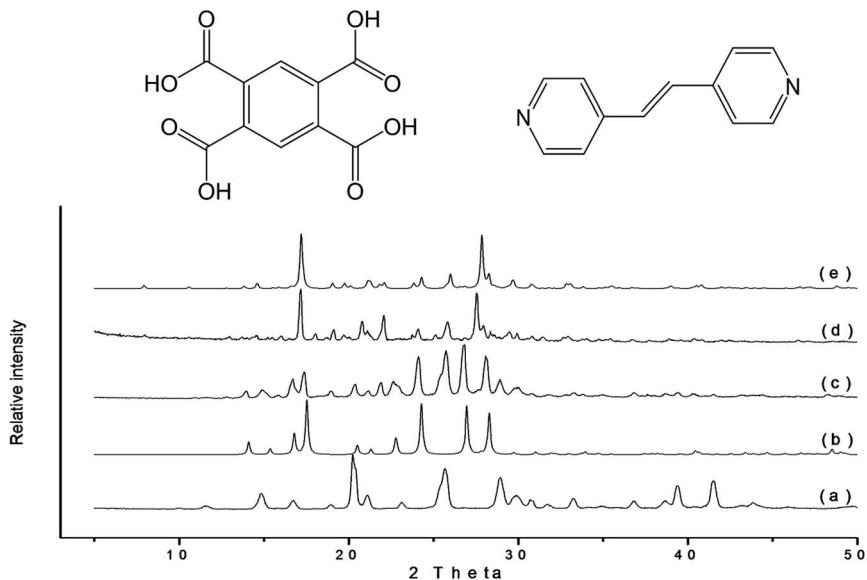
Fig. 15 Demonstration of the enhanced kinetics of cocystal formation upon addition of a few drops of methanol to the grinding jar. PXRD patterns for (a) tetracarboxylic acid, (b) bipirydil, (c) outcome of neat grinding for 60 minutes (as the sum of the reactants), (d) the product obtained when a few drops of methanol are added and (e) the simulated pattern for the cocystal.
