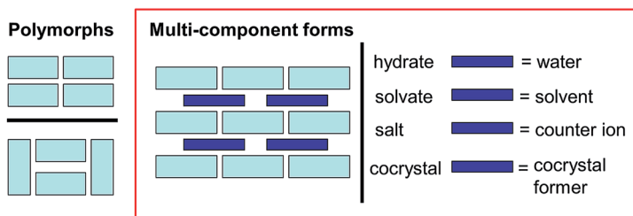
Fig. 9 Schematic of the characteristics of polymorphs and multicomponent systems. Cocystals represent a sub-set of the multicomponent group, frequently that characterised by the requirement that the components be neutral and solid at room temperature.
