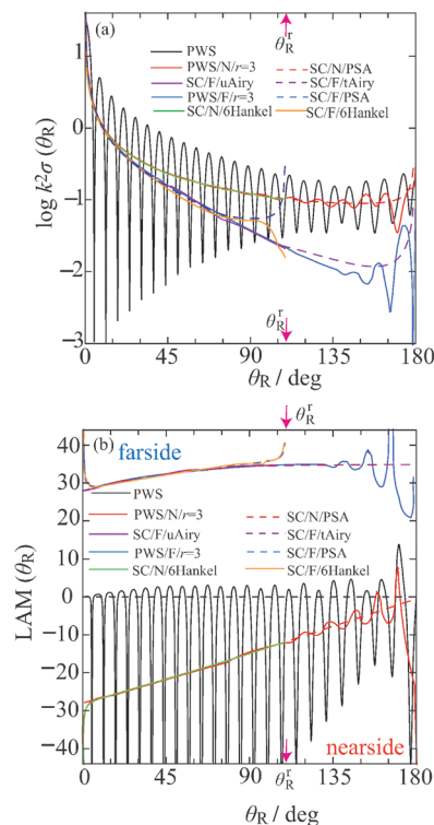
Fig. 4 Nearside–farside analyses for the dimensionless logarithmic angular distribution and the Local Angular Momentum. Black solid curve: PWS. Red solid curve: \text{PWS/N}/r = 3 . Red dashed curve: \text{SC/N/PSA} . Solid purple curve: \text{SC/F}/u\text{Airy} . Purple dashed curve: \text{SC/F}/t\text{Airy} . Blue solid curve: \text{PWS/F}/r = 3 . Blue dashed curve: \text{SC/F/PSA} . Green solid curve: \text{SC/N}/6\text{Hankel} . Orange solid curve: \text{SC/F}/6\text{Hankel} . The pink solid arrows indicate the rainbow angle, \theta_R^r = 109.2^\circ . (a) Full and NF \log k^2\sigma(\theta_R) versus \theta_R . (b) Full and NF \text{LAM}(\theta_R) versus \theta_R .
