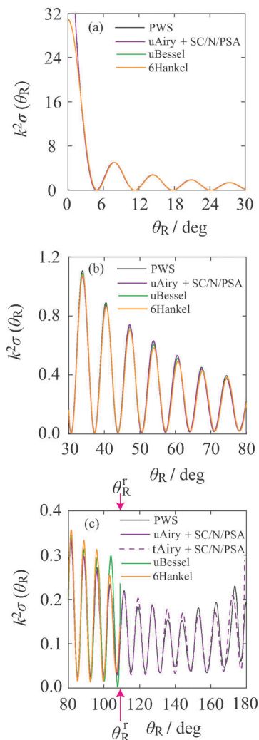
Fig. 3 Linear plot of the dimensionless angular distribution, k^2\sigma(\theta_R) versus \theta_R . Black solid curve: PWS. Purple solid curve: u\text{Airy} + \text{SC/N/PSA} . Purple dashed curve: t\text{Airy} + \text{SC/N/PSA} . Green solid curve: u\text{Bessel} . Orange solid curve: 6\text{Hankel} . (a) 0^\circ \leq \theta_R \leq 30^\circ . The u\text{Airy} + \text{SC/N/PSA} curve diverges as \theta_R \rightarrow 0^\circ . (b) 30^\circ \leq \theta_R \leq 80^\circ . The PWS and u\text{Airy} + \text{SC/N/PSA} curves are almost coincident for \theta_R \geq 35^\circ . (c) 80^\circ \leq \theta_R \leq 180^\circ . The pink solid arrows indicate the rainbow angle, \theta_R^r = 109.2^\circ . The u\text{Bessel} curve diverges as \theta_R \rightarrow \theta_R^r . The t\text{Airy} + \text{SC/N/PSA} approximation is used for \theta_R \geq \theta_R^r ; it diverges as \theta_R \rightarrow 180^\circ .
