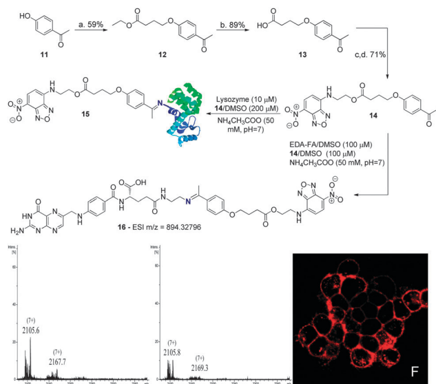
Scheme 5 (a) Ethyl 4-bromobutyrate, K 2 CO 3 , NaI, acetone, reflux, 20 h; (b) TFA, H 2 O, 90 °C, 3 h; (c) DMAP, EDC; DCM, 0 °C, 1 h; (d) NBDNH(CH 2 ) 2 OH, DCM, rt, 5 h. UV spectrum: see ESI† for compound 14. Reaction of lysozyme (10 μM) with 14 (200 μM) in acetate buffer (50 mM, pH 7) at room temperature. Zoom of the (7+) charge state of the ESI-FTICR-MS spectra after 30 min and 2 h of reaction. Image F shows NCI-H460 treated with compound 16. Incubation and imaging conditions are likewise described in Scheme 3.
