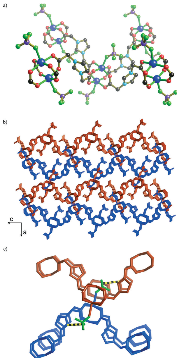
Fig. 2 The structure of [\text{Cu}_2(\text{imdc})_2(\text{BF}_4)_2] (2) showing: a) part of the undulating [\text{Cu}_2(\text{imdc})_2(\text{BF}_4)_2] square grid sheet in which \text{Cu}_2 units are bridged by \text{imdc}^- anions; coordinate bonds are indicated by green connections, atom colour code: Cu – deep blue, F – green, O – red, N – light blue, C – black, B – purple b) a stick representation indicating the relative arrangement of the 2D networks viewed almost normal to the stacking direction (along the a axis); c) the C–H...F hydrogen bonding interaction, indicated by yellow and black striped connections, between sheets involving the coordinated \text{BF}_4^- anion and an imidazolium proton; \text{BF}_4^- anions are represented by green connections. Hydrogen atoms have been removed for clarity.
