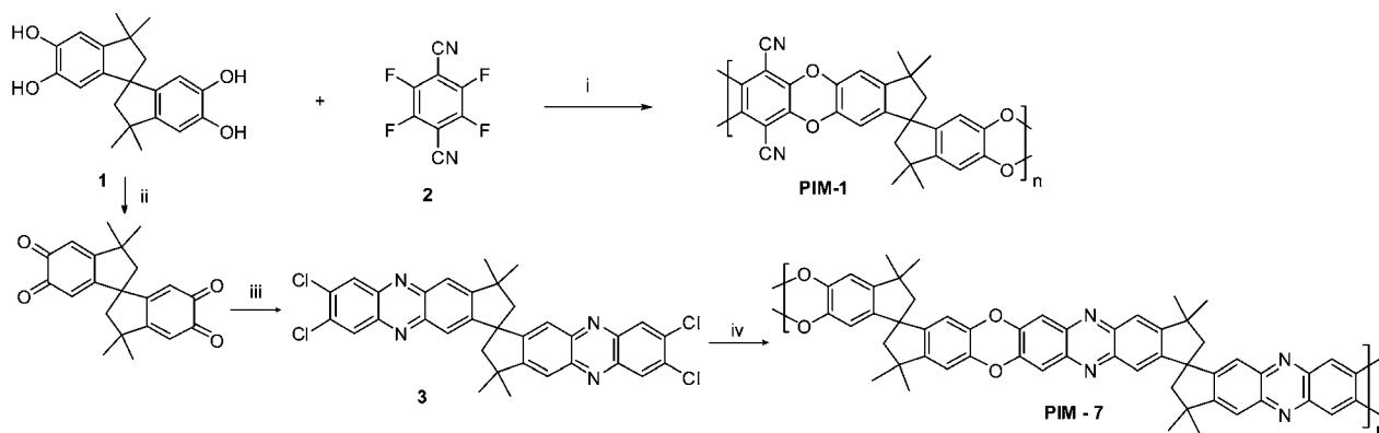
Scheme 1 Synthesis of PIM-1 and PIM-7. Reagents and conditions: (i) \text{K}_2\text{CO}_3 , DMF, 65 °C, 48 h; (ii) nitric acid, AcOH, \text{C}_2\text{H}_5\text{OH} , 0 °C, 24 h; (iii) 4,5-dichloro-1,2-diaminobenzene, AcOH, reflux, 3 h; (iv) bis(catechol) (A), \text{K}_2\text{CO}_3 , 18-crown-6, DMF, 150 °C, 48 h.
