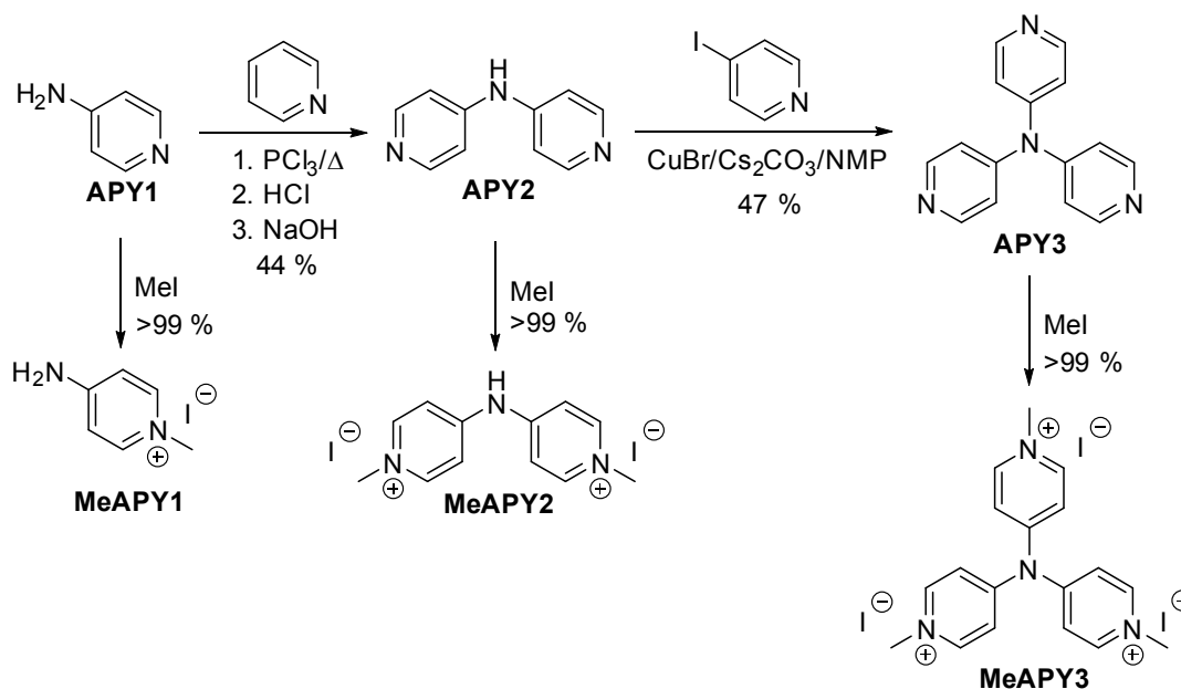
Scheme 1 Synthesis of aminopyridines (APY) and aminopyridiniums (MeAPY)
