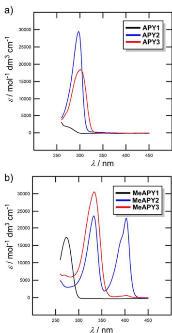
Fig. 3 UV/Vis absorption spectra of APY1-3 (a) and MeAPY1-3 (b) measured in DMSO ( c = 2 \times 10^{-5} M)
