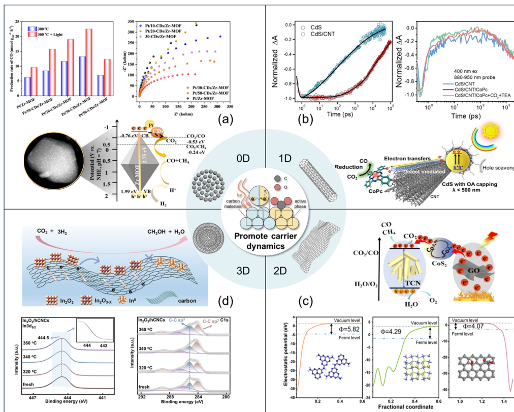
Fig. 5 Carbon-based functional phases for promoting the electron generation and transfer of carriers: (a) effect of CD content on carrier generation and transfer efficiency in Pt/CDs/Zr-MOF. Reproduced with permission. 32 Copyright 2025, Elsevier. (b) Effect of CNTs on carrier separation and transfer in CdS/CNT/CoPc. Reproduced with permission. 33 Copyright 2023, John Wiley & Sons. (c) Effect of graphene on carrier generation in GO/CoS 2 /TCN. Reproduced with permission. 99 Copyright 2025, Elsevier. (d) Effect of hCNCs on carrier transfer in In 2 O 3 /hCNCs. Reproduced with permission. 72 Copyright 2025, American Chemical Society.
