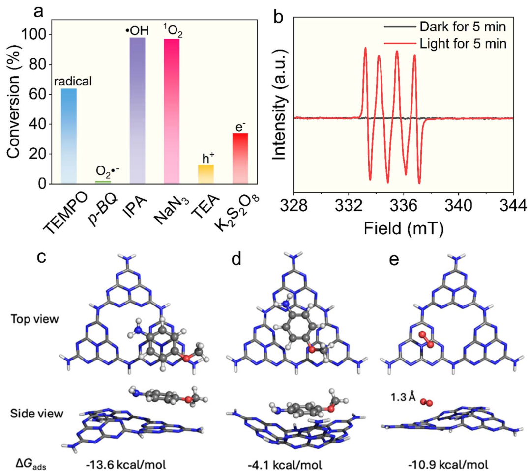
Fig. 5 (a) Scavenger study and (b) EPR spectrum of the DMPO–superoxide radical. Theoretical calculations for the adsorption of p -anisidine and the activation of O_2 on the mpq- C_3N_4 photocatalyst associated with the corresponding adsorption Gibbs energies ( \Delta G_{ads} ): (c) p -anisidine on mpq- C_3N_4 (site 1), (d) p -anisidine on mpq- C_3N_4 (site 2), and (e) superoxide radical on mpq- C_3N_4 . The O–O bond lengths in Å show the activation of O_2 and the formation of superoxide radicals. Nitrogen is shown in blue, carbon in grey, oxygen in red, and hydrogen in white.
