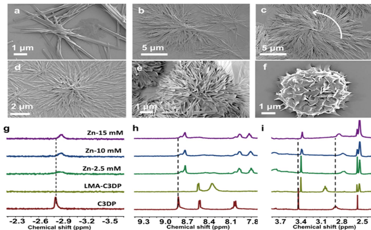
Fig. 3 SEM images of C3DP-LMA-Zn assemblies with increasing concentration of \text{Zn}(\text{II}) : (a) 0 mM, (b) 2.5 mM, (c) 5 mM, (d) 7 mM, (e) 12.5 mM and (f) 14.5 mM. (g–i) ^1\text{H} NMR titration of C3DP in \text{DMSO}-d_6 with stepwise and sequential addition of MA in \text{D}_2\text{O} followed by \text{Zn}(\text{OAc})_2 in \text{D}_2\text{O} .
