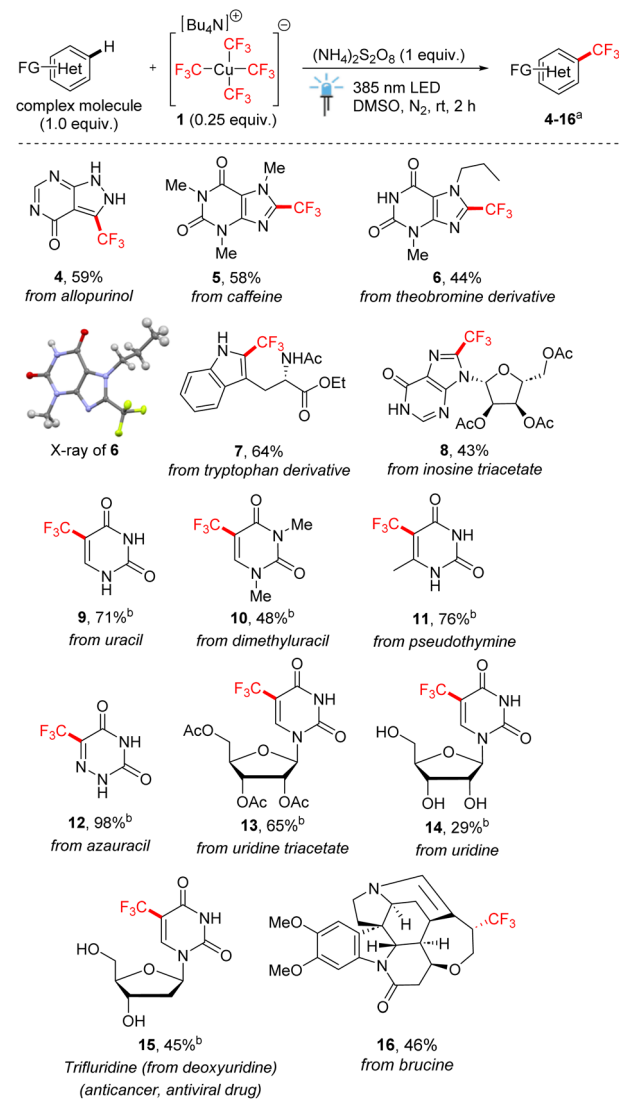
Scheme 3 Late-stage trifluoromethylation of complex heterocycles with 1 (0.25 equiv.). a Isolated yields after column chromatography. b \text{DMSO}/\text{H}_2\text{O} (3:1) as the solvent and \text{Na}_2\text{S}_2\text{O}_8 as the oxidant.
