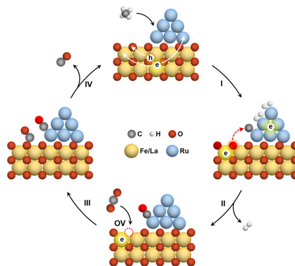
Fig. 6 Illustration of the proposed photothermal DRM mechanism over \text{Ru}/\text{LaFeO}_3 .
