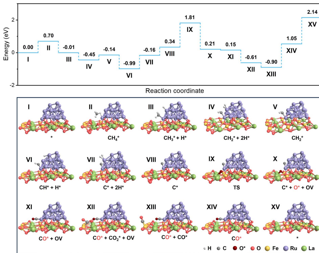
Fig. 5 Relative energy diagrams of \text{CH}_4 and \text{CO}_2 conversion on \text{Ru}/\text{LaFeO}_3 simulated by DFT calculation and some corresponding structures of the key reaction intermediates during the \text{CH}_4 dissociation and \text{CO}_2 conversion processes.
