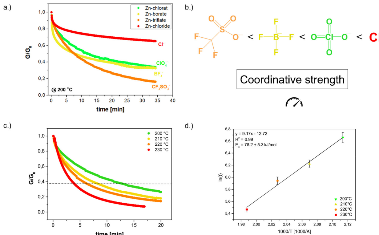
Fig. 3 (a) Stress relaxation measurements at 200 °C with various \text{Zn}^{2+} salts; (b) structures and coordination strengths of the anions used; (c) stress relaxation measurements of a sample containing 5 mol% zinc at different temperatures and (d) Arrhenius plot derived from these measurements.
