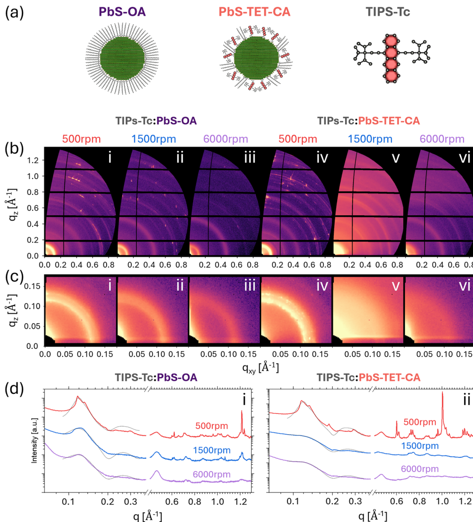
Fig. 1 (a) Illustration of PbS QDs possessing either oleic acid (PbS-OA) or tetracene carboxylic acid (PbS-TET-CA) ligands and small molecule host, TIPS-tetracene (TIPS-Tc). (b) and (c) 2D GIXS data of (i, ii, iii) TIPS-Tc:PbS-OA and (iv, v, vi) TIPS-Tc:PbS-TET-CA OSC:QD blends deposited via spin-coating at speeds of 500 rpm, 1500 rpm and 6000 rpm. (d) Corresponding azimuthally integrated 1D intensity profiles of (i) TIPS-Tc:PbS-OA and (ii) TIPS-Tc:PbS-TET-CA prepared via spin-coating and the associated fits to the GISAXS region (grey lines) using an FCC paracrystal model. The 1D data have been multiplied by an arbitrary coefficient to be shifted along the intensity axis for clarity. Note the peak at q \sim 0.45 \text{ \AA}^{-1} is a background peak from the Kapton window.
