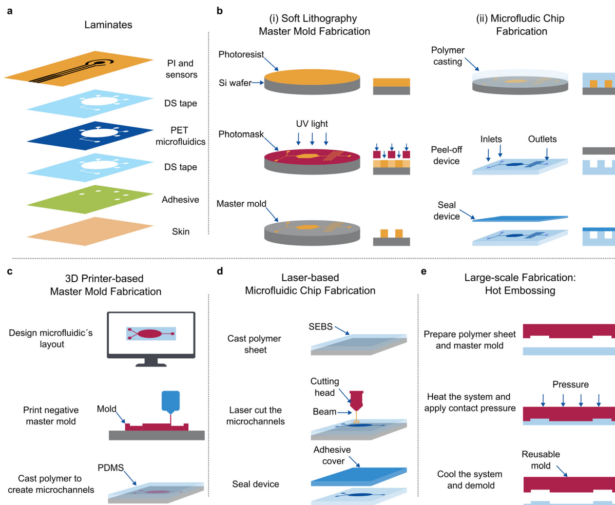
Fig. 7 Fabrication methods for microfluidic wearable biosensors. a) Laminates-based fabrication involves stacking layers from different materials to create the microchannels. PI: polyimide, DS: double-sided tape. b) Soft lithography is used to manufacture master molds for microfluidic fabrication. A polymer is cast on the mold surface and cured, transferring the master features to the polymeric substrate. c) 3D printing can be used to create the master molds avoiding the need for clean room access. However, this method's resolution depends on the printer and is generally low compared to other techniques. d) Laser-based fabrication uses different types of lasers to etch the microchannels into the substrate. This method can also be used to manufacture master molds. e) Hot embossing is a large-scale fabrication which uses a master mold and a thermoplastic to imprint the microfluidic design onto the polymer sheet.
