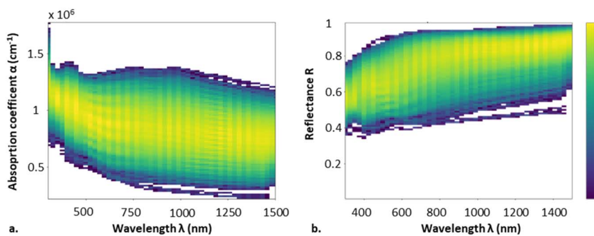
Fig. 7 Calculation of the (a) absorption and (b) reflectance proxy within the 300–1500 nm spectral range, for 10 994 HEAs.
