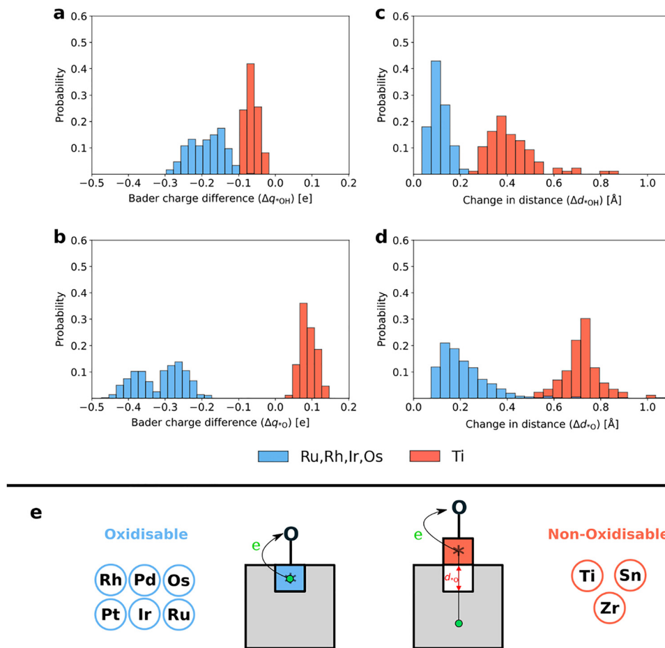
Fig. 3 Probability distributions of the Bader charge difference ( \Delta q_{\text{A}} ) at the adsorption site atom in the RuRhIrOsTi high entropy oxides dataset after (a) \text{*OH} , and (b) \text{*O} adsorption. (c) Probability distributions of the change in the distance ( \Delta d_{\text{A}} ) between the adsorption site atom and the oxygen atom underneath after \text{*OH} and (d) \text{*O} adsorption. Data for Ru, Rh, Ir, and Os adsorption sites are aggregated into a single distribution for comparison with the distribution based on data for Ti sites. (e) Schematic figure of the proposed explanation for the different adsorption energies trends observed for Ti, Sn, and Zr guests and Ru, Rh, Ir, Os, Pd, and Pt guests.
