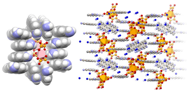
Fig. 7 \pi -Stacking of [HPF] + cations in crystalline [HPF] 3 [Ga(ox) 3 ] 2 ·4H 2 O (left), and encapsulation of two [Ga(ox) 3 ] 3- anions within a proflavium-cation envelope (right). Reproduced from ref. 111.
