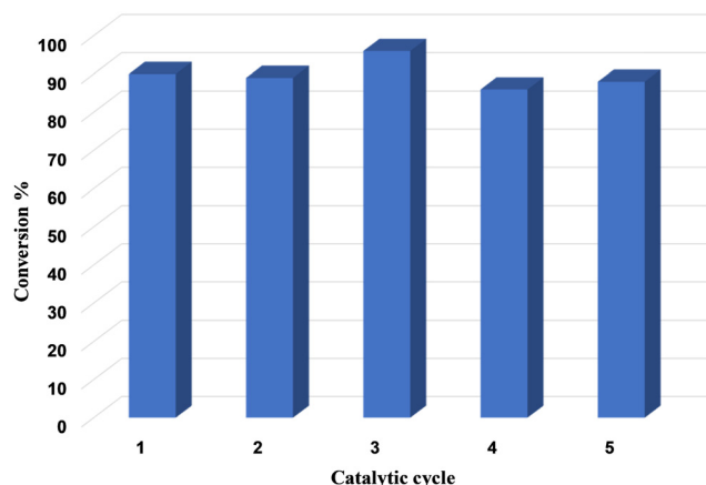
Fig. 2 Reusability of \text{N}(\text{Me})_3^+\text{-P5} for multi-cycloaddition cycles using ECH as a substrate; see Fig. S19 (ESI†).
