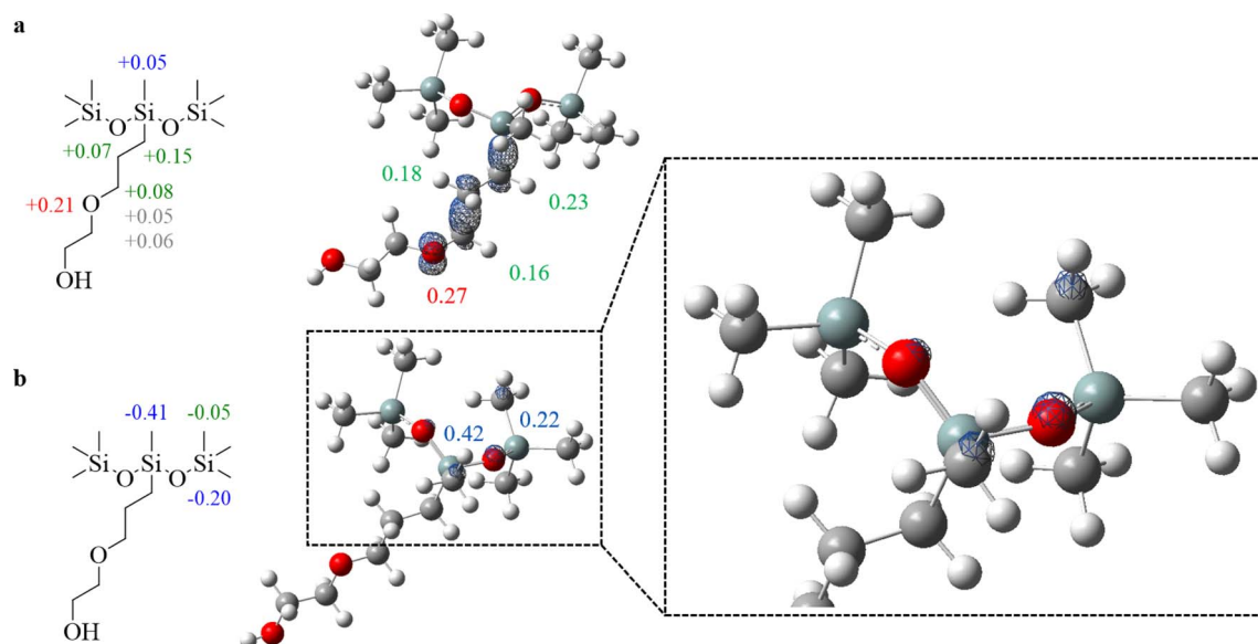
Fig. 5 Change in partial atomic charges (left) and spin density isosurfaces (right) for (a) oxidized and (b) reduced TriSiI-1n. Green values correspond to carbon, red correspond to oxygen, blue correspond to silicon, and grey corresponds to hydrogen. Positive values indicate a decrease in charge. In the isosurfaces, oxygen atoms are red, silicon atoms are pale blue, carbon atoms are gray, and hydrogen atoms are white. All values are presented in a.u. and only spin densities greater than 0.15 a.u. and changes in partial atomic charge greater than 0.05 a.u. are reported. The isovalues for (a) and (b) are 0.01 and 0.0035, respectively. NBO analysis was computed at the \omega b97X-D/6-311+G(2d,2p) level of theory with SMD water solvation.
