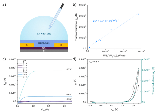
Fig. 5 (a) Schematic of the MEEA-SiPc OECT. (b) Determination of \mu C^* from the plot of g_m vs. WdL^{-1}(V_{\text{GS}} - V_T) . Characteristic (c) output and (d) transfer curves of MEEA-SiPc OECTs in 0.1 M NaCl with W = 10\,000 \mu\text{m} , L = 2.5 \mu\text{m} .
