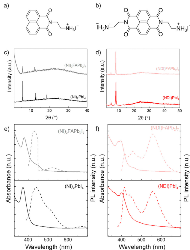
Fig. 1 Structural and optoelectronic properties of naphthal(enedi)imide LD perovskites. (a) and (b) Structural representations of NI and NDI. (c) and (d) XRD patterns of films of (c) (NI)_2PbI_4 , (NI)_2FAPb_2I_7 , (d) (NDI)PbI_4 , and (NDI)FAPb_2I_7 nominal compositions. (e) and (f) UV-Vis (full line) and PL (dashed line) spectra of films based on (e) (NI)_2PbI_4 , (NI)_2FAPb_2I_7 , (f) (NDI)PbI_4 , and (NDI)FAPb_2I_7 nominal compositions on glass.
