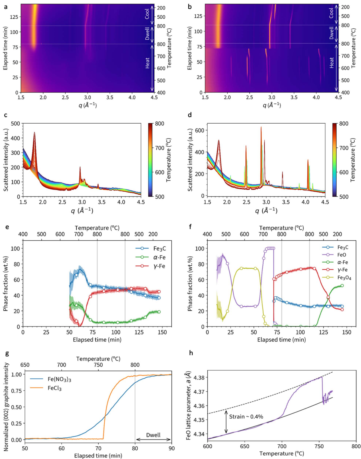
Fig. 2 Heatmaps of WAXS data for samples of (a) cellulose + Fe(NO 3 ) 3 and (b) cellulose + FeCl 3 heated to 800 ^{\circ}\text{C} under nitrogen. Also diffraction data for (c) cellulose + Fe(NO 3 ) 3 and (d) cellulose + FeCl 3 with an additional panel showing the temperature for each pattern during heating to 800 ^{\circ}\text{C} . Phase fractions extracted from Rietveld refinement of data for (e) cellulose + Fe(NO 3 ) 3 and (f) cellulose + FeCl 3 . A plot of (g) normalised graphite (002) peak intensity vs. time and temperature. (h) Plot showing expansion of FeO lattice parameter a with increasing temperature.
