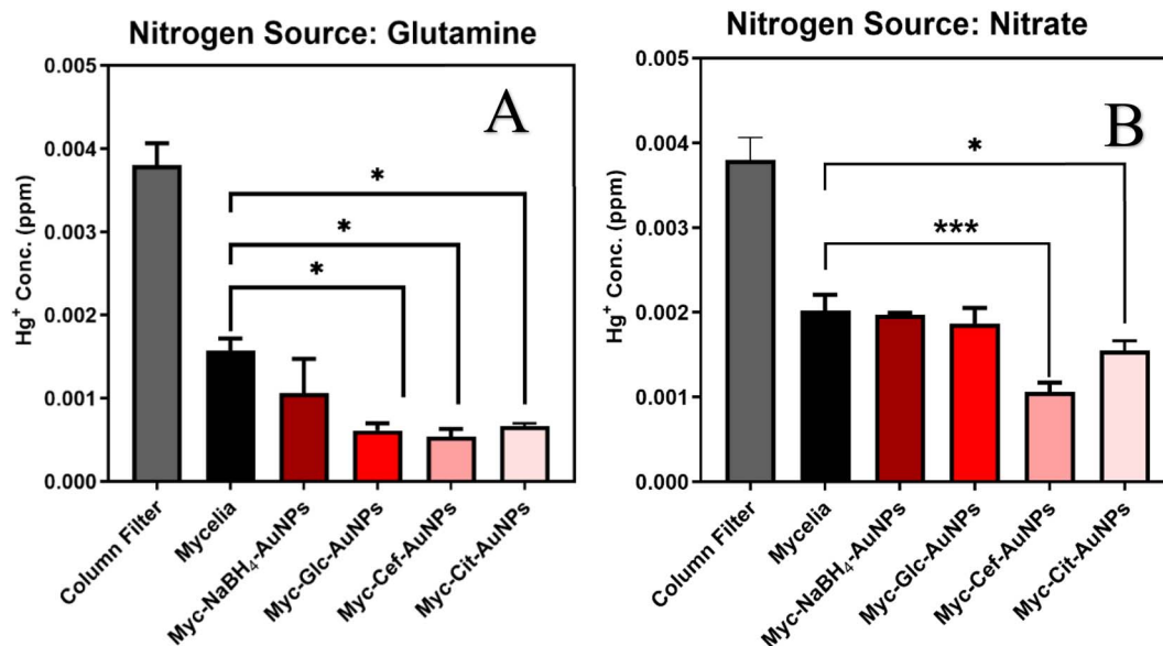
Fig. 6 Quantitative comparison of Hg 2+ removed by Aspergillus niger mycelia after 30 minutes of interaction at 30 µg mL -1 when either glutamine (A) or nitrate (B) was used as a nitrogen source in the growth of the mycelia. The level of significance: *( p \leq 0.05 ), **( p \leq 0.01 ), and ***( P \leq 0.001 ). The starting level of mercury is 5 ppb.
