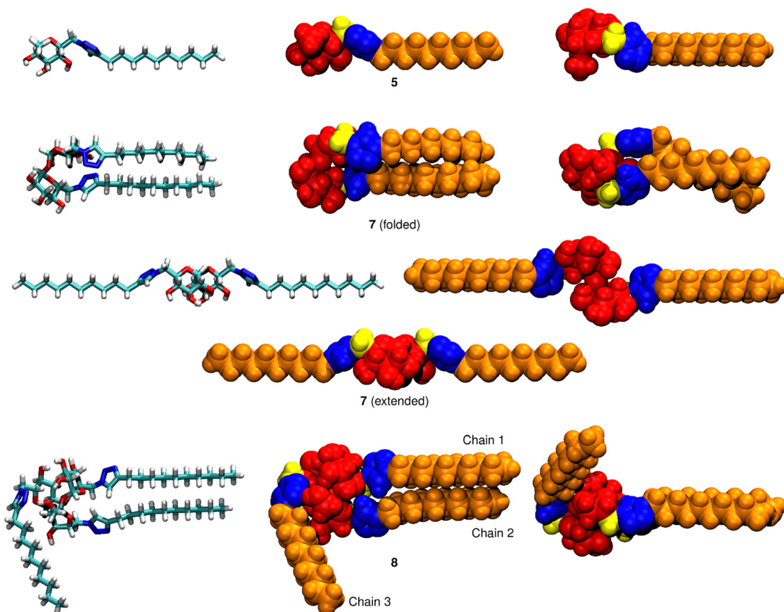
Fig. 5 Examples of optimised structures of 5 , 7 in folded and extended forms, and 8 , determined at the \omega\text{B97X-D/cc-pVDZ} level of theory. The structures shown as van der Waals surfaces (centre and right-hand columns) are coloured according to moiety types: sugar (red), triazole (blue), alkyl chain (orange), and sugar–triazole methylene ( \text{CH}_2 ) linking group (yellow). The left-hand and centre columns show the same orientations, and the right-hand column shows horizontally rotated views.
