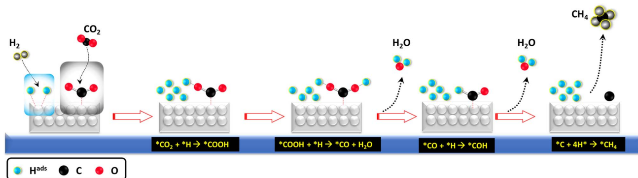
Fig. 5 The carboxyl pathway of \text{CO}_2 methanation.
