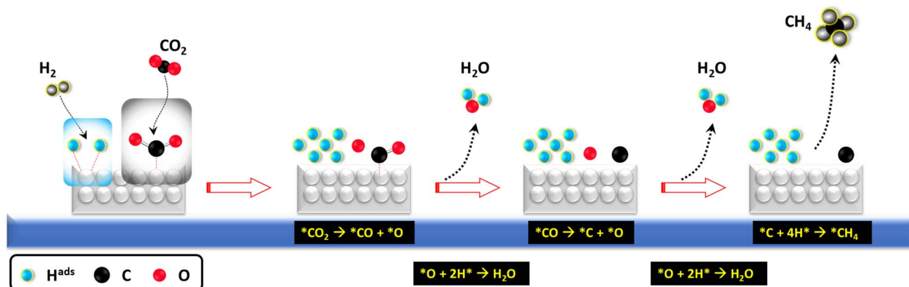
Fig. 6 The dissociative reaction pathway of \text{CO}_2 methanation.
