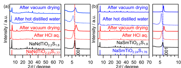
Fig. 6 XRD patterns of the sulfurized products, \text{NaMTiO}_{2.2}\text{S}_{1.8} ( M = (a) \text{Nd} , (b) \text{Sm} ) and the samples after stirring under dark conditions in an \text{HCl} aqueous solution for 24 h or hot distilled water for 72 h, followed by vacuum drying, along with the reference patterns of \text{NaNdTiO}_{2.23}\text{S}_{1.77} (this work) and \text{NaSmTiO}_{2.24}\text{S}_{1.76} (this work).
