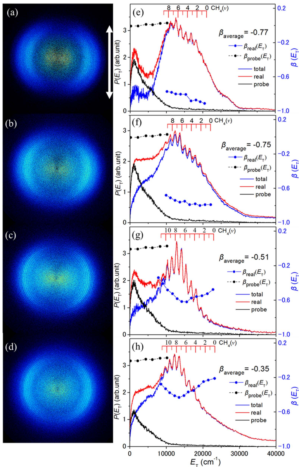
Fig. 5 TS-VM images of the S^1D fragments formed by photolysis of jet-cooled CH_3SH molecules at \lambda = (a) 204, (b) 199, (c) 196 and (d) 193 nm, with \epsilon_{\text{phot}} aligned vertically in the plane of the image as indicated by the double headed arrow in (a). Panels (e)–(h) show the P(E_T) distributions derived from each two-colour image (red trace), from the 130.091 nm probe-laser only image (black trace) and the ‘real’ pump–probe two-colour P(E_T) distribution obtained from the difference (blue trace), referenced to the left-hand y-axis scale. The black and blue dots show the \beta(E_T) distributions derived from the corresponding traces, referenced to the right-hand y-axis scale. The \beta_{\text{average}} value for the signal from photolysis laser induced dissociation determined over the indicated E_T range is also included in the inset. The red combs in panels (c) and (d) show the maximum E_T values for different S^1D + CH_4(v_4) product channels.
