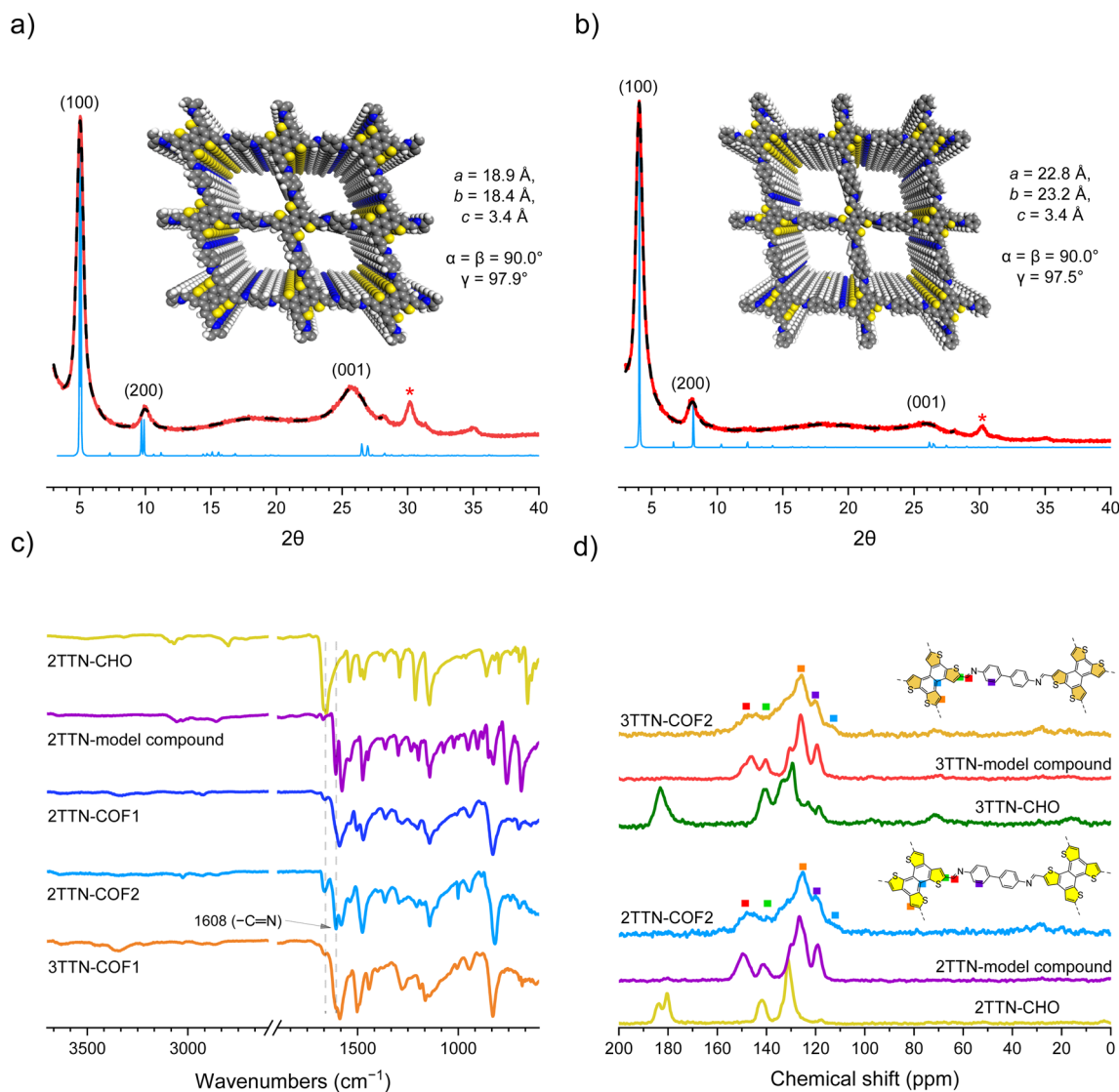
Fig. 1 PXRD patterns of (a) 2TTN-COF1 powder (observed (red), refined (dashed) and simulated AA stacking (blue), R_p = 2.15\% , R_{wp} = 2.74\% ), (b) 2TTN-COF2 (observed (red), refined (dashed) and simulated AA stacking (blue), R_p = 2.55\% , R_{wp} = 3.45\% ), and the inset shows the simulated structures. Full Width at Half Maximum (FWHM) is 0.57^\circ and 0.56^\circ for 2TTN-COF1 and 2TTN-COF2, compared to 0.85^\circ and 0.63^\circ for 3TTN-COF1 and 3TTN-COF2 for 100 plane peaks, respectively (Fig. S3). (c) IR spectra of aldehydes, the model compound, and COF powders showing the imine linkages at 1608\text{ cm}^{-1} and residual aldehyde peak at 1660\text{ cm}^{-1} , and (d) comparison of ^{13}\text{C} NMR starting materials, model compounds and COF powders measured at (CP-MAS, 13 kHz). The peaks marked by * in (a) and (b) are due to trace amounts of zirconia leaching from jars ( \leq 0.5\% based on X-ray photoelectron spectroscopy (XPS), Fig. S6b, S9–S13).
