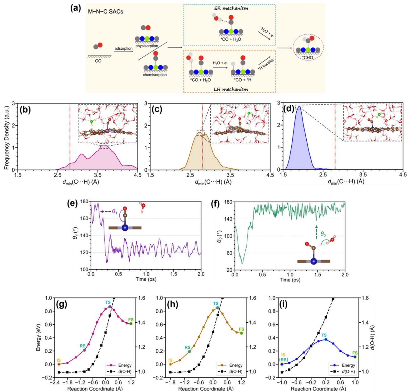
Fig. 10 (a) Schematic diagram of the mechanistic pathways of CO reduction to \text{*CHO} via the ER and LH mechanisms on M-N-C SACs. 117 (b)–(d) Frequency density distribution of d_{\text{min}}(\text{C}\cdots\text{H}) for (b) [\text{MnPc}]^{2-} , (c) [\text{FePc}]^{2-} , and (d) [\text{CoPc}]^{2-} in explicit water, respectively. The red dashed lines indicate a d_{\text{min}}(\text{C}\cdots\text{H}) of 2.84 Å. Representative snapshots from the trajectory are presented, showing instances in which d_{\text{min}}(\text{C}\cdots\text{H}) aligns with the peak of the frequency density. The \text{H}_2\text{O} closest to \text{*CO} is highlighted. (e) and (f) The evolution of the Co–C–O angle ( \theta_1 ) and the C...H–O angle ( \theta_2 ) during the first 2 ps of the molecular dynamics simulation. Snapshots of the Co atom with \text{*CO} and the closest \text{H}_2\text{O} are included, corresponding to the simulation time indicated by the arrowheads. (g)–(i) Free energy profile and evolution of average d(\text{O}-\text{H}) along the reaction coordinate for (g) FePc, (h) MnPc, and (i) CoPc systems. The reaction coordinate is quantified by the collective variable of \xi = d(\text{O}-\text{H}) - d(\text{C}-\text{H}) . 119 Reproduced from ref. 117 and 119 with permission from American Chemical Society, copyright 2023, 2024.
