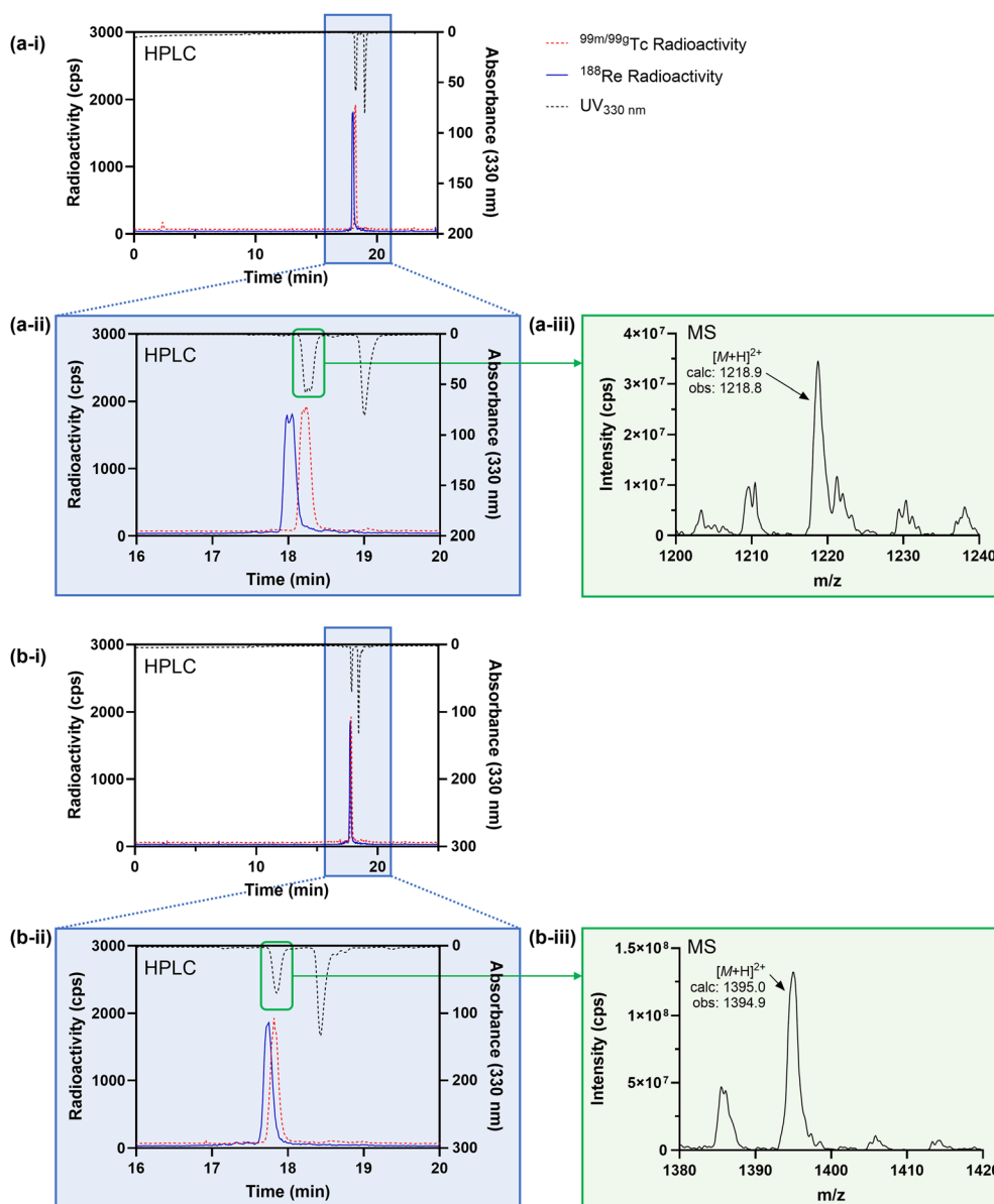
Fig. 5 (a-i) and (a-ii) UV chromatogram and radiochromatograms of reactions containing [\text{MO}_2(\text{DP}^{\text{An}}\text{-PSMAT})_2]^+ ( M = {}^{99\text{m}}\text{Tc} , {}^{99\text{g}}\text{Tc} or {}^{188}\text{Re} ); (a-iii) mass spectrum showing signal corresponding to [{}^{99\text{g}}\text{TcO}_2(\text{DP}^{\text{An}}\text{-PSMAT})_2]^+ . (b-i and b-ii) UV chromatogram and radiochromatograms of reactions containing [\text{MO}_2(\text{DP}^{\text{MEP}}\text{-PSMAT})_2]^+ ( M = {}^{99\text{g}}\text{Tc} , {}^{99\text{m}}\text{Tc} or {}^{188}\text{Re} ); (b-iii) mass spectrum showing signal corresponding to [{}^{99\text{g}}\text{TcO}_2(\text{DP}^{\text{MEP}}\text{-PSMAT})_2]^+ .
